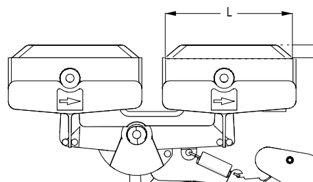
Illustration of conductor contact length and wear height 081508, 081509
